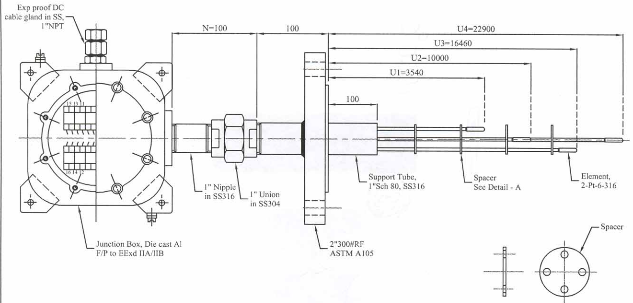
Detail-A (Spacer)
